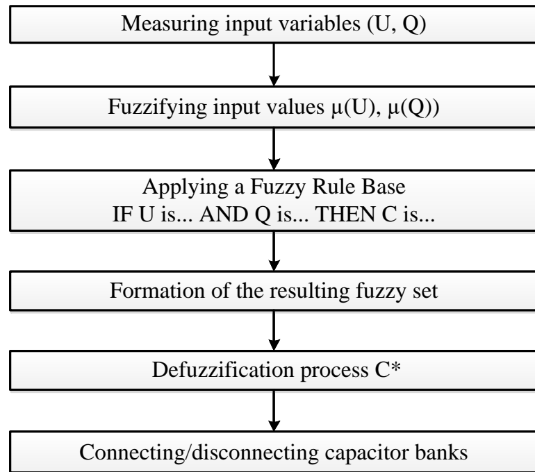
Figure 1. Algorithm for automatic control of reactive power at industrial enterprises based on fuzzy logic
